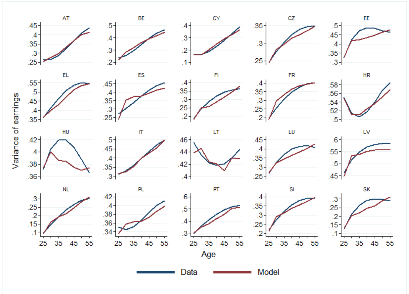
Figure 27: Model fit
