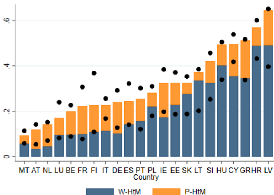
Figure 19: HtM sensitivity
